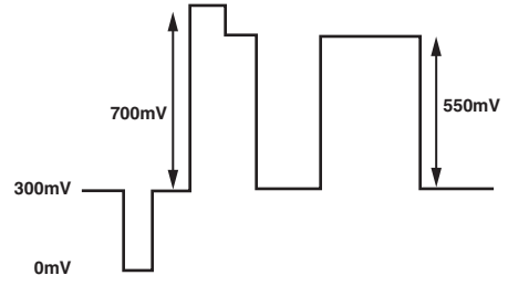
Figure 99. SD RGB Output Levels—RGB Sync Enabled
